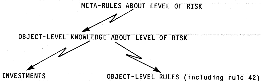
Figure 12 -- Applying meta-level knowledge in two ways
